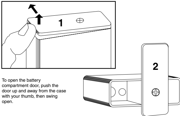
Figure 5 - Battery Replacement
